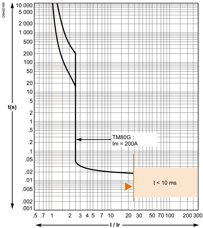
TM80G
