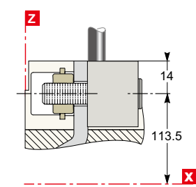
DB115454 CVS400/630
