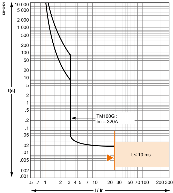
TM100G
