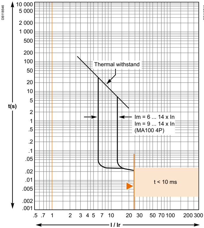
MA2.5... MA100
