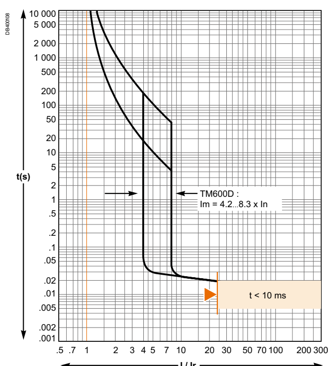
TM600D
