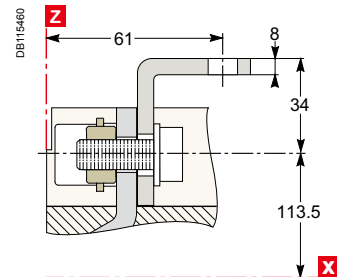
DB115460 CVS400/630
