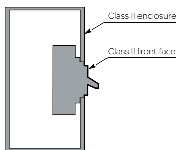
Class II panel with circuit breaker having a class II front face
